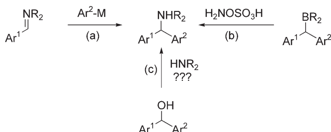
Scheme 1. Synthesis of diarylamines.
