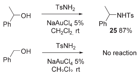
Scheme 5. Amination of alkylarylmethyl alcohols.
