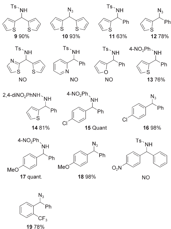
Scheme 3. Gold-catalyzed amination on various aromatic and heteroaromatic substrates. NO: not obtained.
